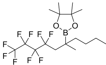
4,4,5,5-Tetramethyl-2-(7,7,8,8,9,9,10,10,10-nonafluoro-5-methyldecyl-5-yl)-1,3,2-dioxaborolane
